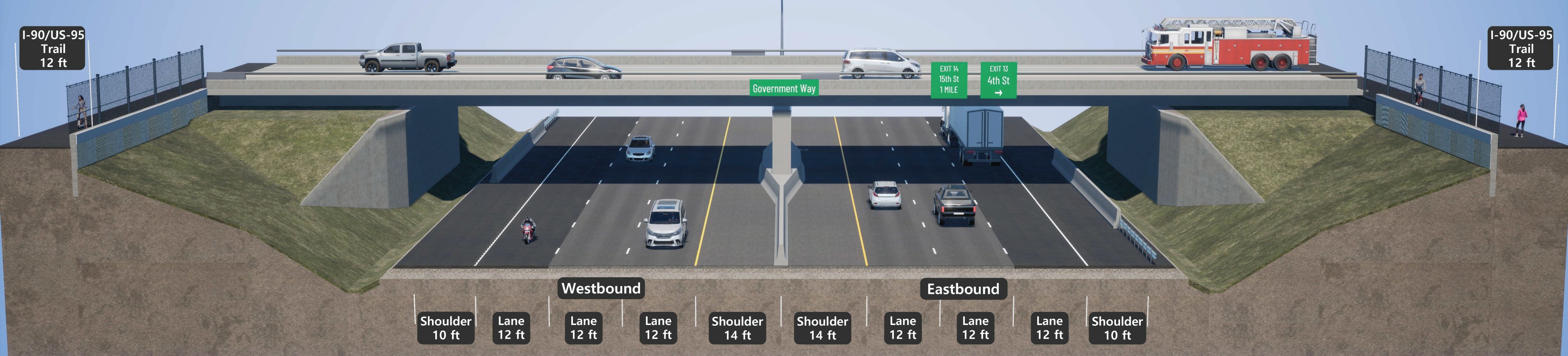
I-90 Typical Section between US-95 and 4th Street (Looking East)
