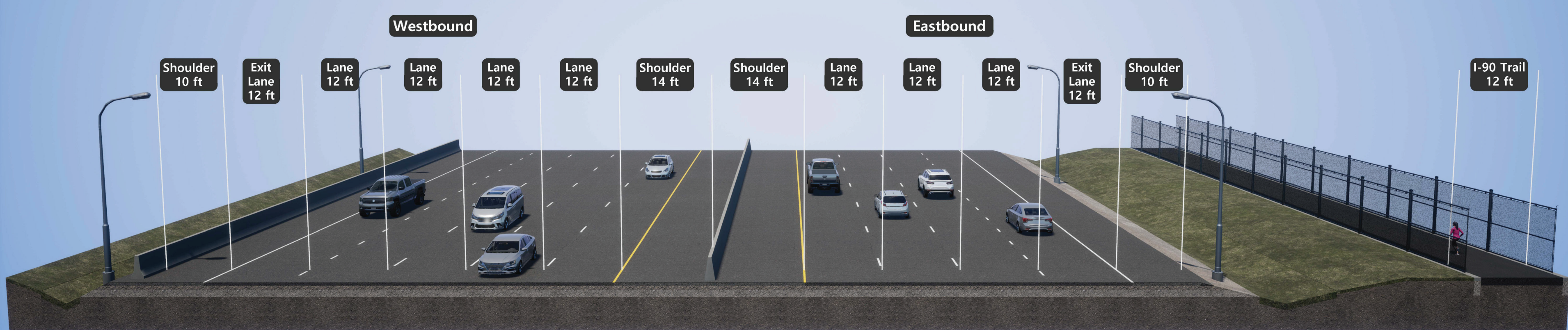
I-90 Typical Section between Northwest Boulevard and US-95 (Looking East)
